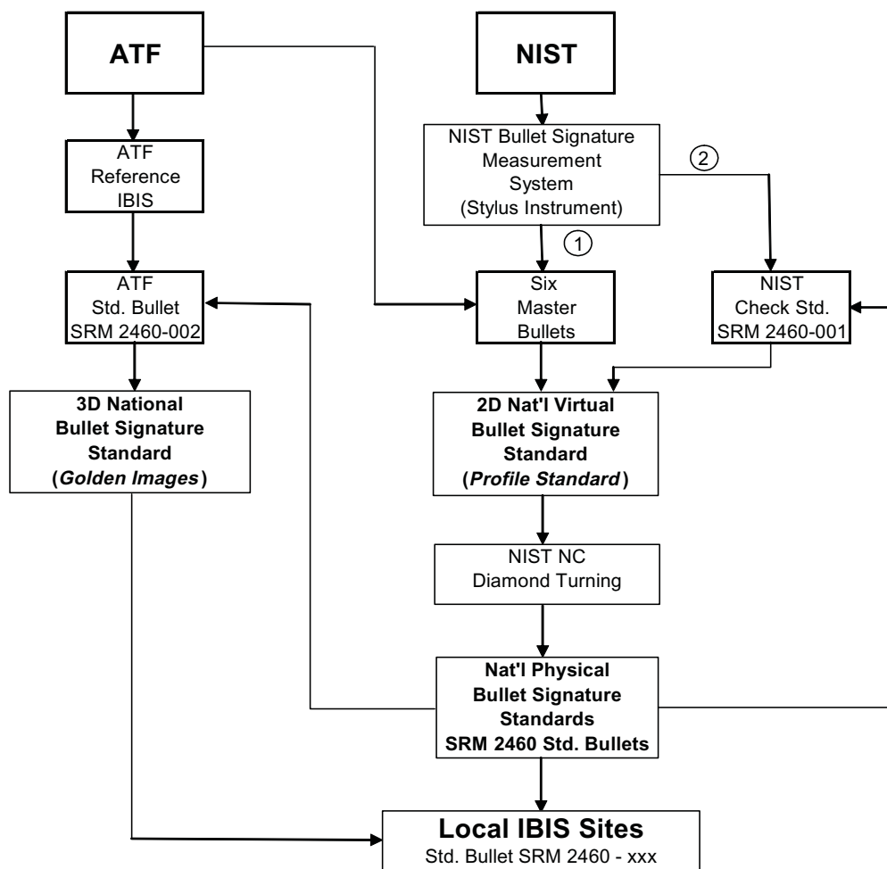
Fig. 2. Establishment of a Traceability and Quality System for NIST's Topography Measurements and NIBIN's Acquisitions and Correlations of Ballistics Signatures
